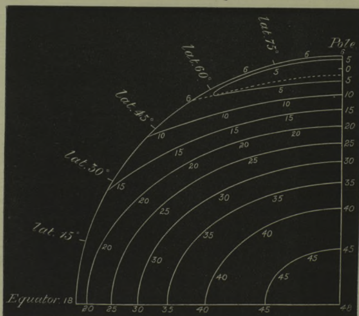
Diagram showing curves of equal Stress-difference due to the weight of 2nd harmonic inequalities or to tide-generating force.
